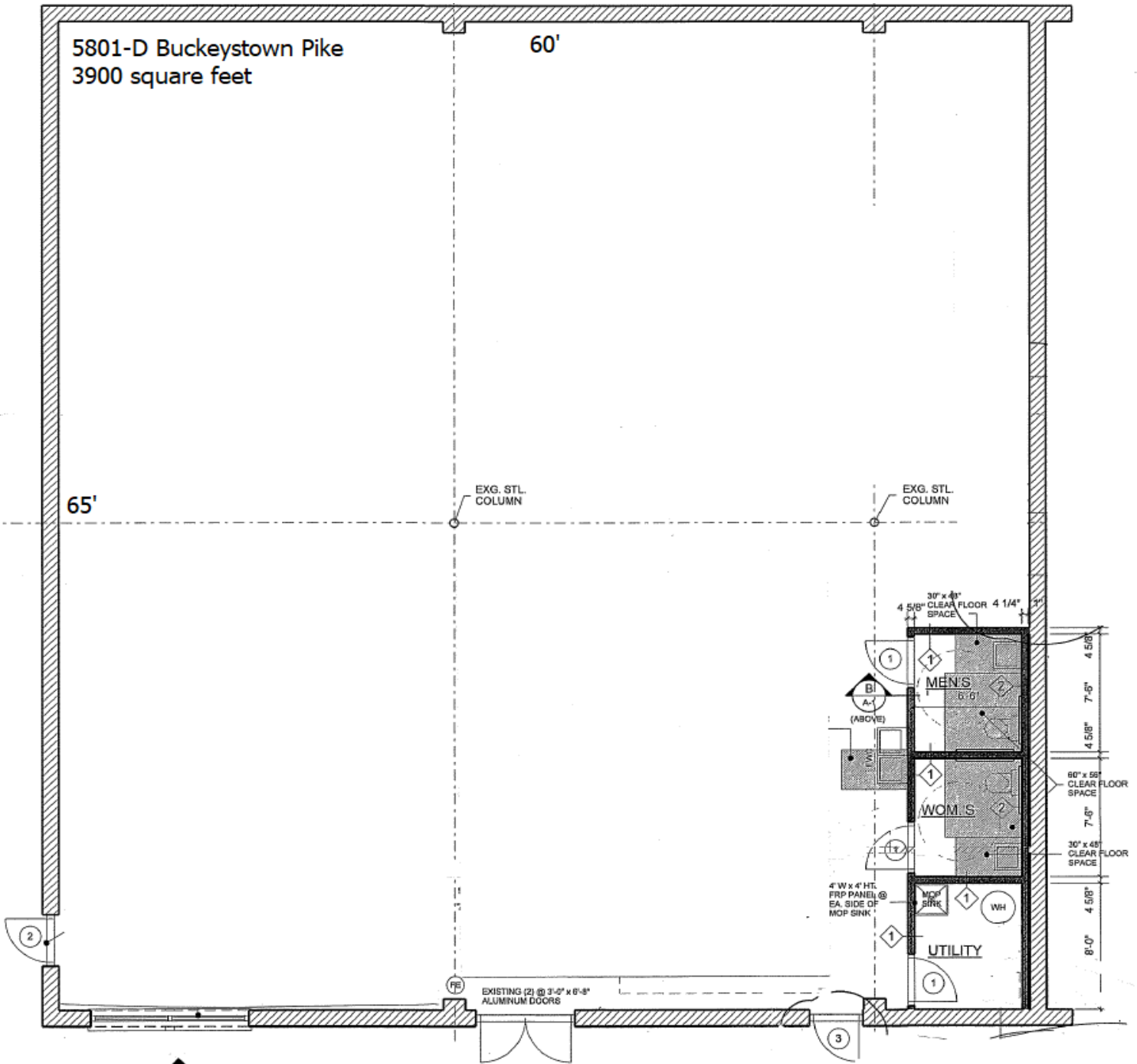
1 A-1 EXISTING FLOOR PLAN
